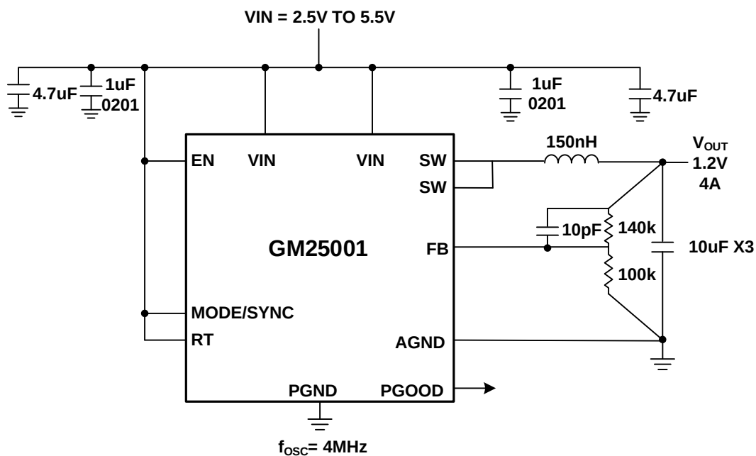
图 30. 4MHz, V IN =3.3V, V OUT =1.2V, I LOAD =4A
