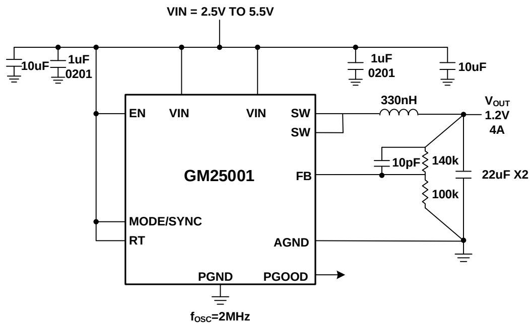
图 29. 2MHz, V IN =3.3V, V OUT =1.2V, I LOAD =4A
