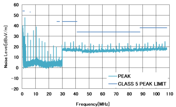
图 29. GM2500_DEMOZ CISPR25 Conducted Emission with Class 5 Peak Limits (Voltage Method)
