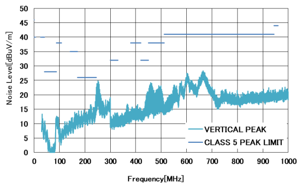
图 31. GM2500_DEMOZ CISPR25 Radiated Emission (Vertical)
