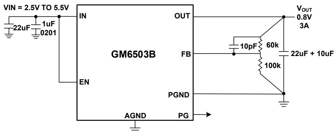
图 17. V IN =3.3V, V OUT =0.8V, I LOAD =3A
