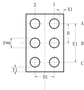
TOP VIEW (BALL SIDE UP)
