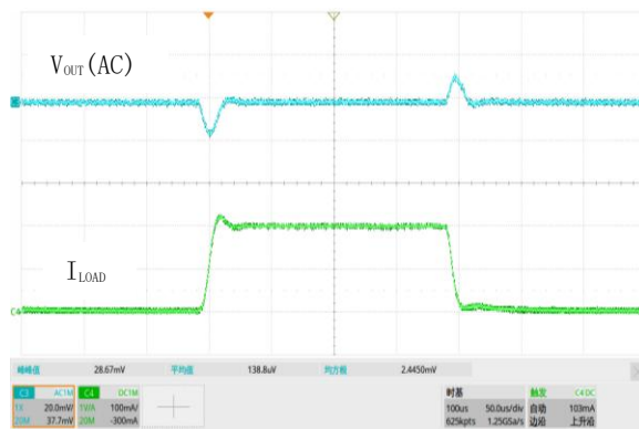
图 24. 负载瞬态响应, V_{IN}=4.3V , V_{OUT}=3.3V , I_{OUT}=1mA to 200mA
