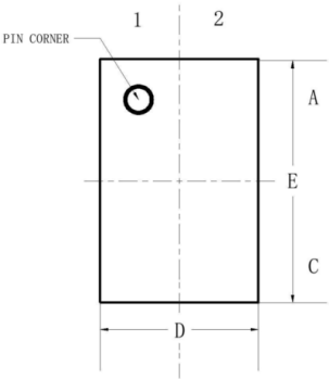
BOTTOM VIEW (BALL SIDE DOWN)
