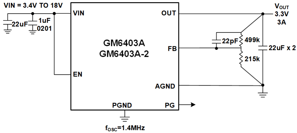
图 17. V IN =12V, V OUT =3.3V, I LOAD =3A, FB=1V
