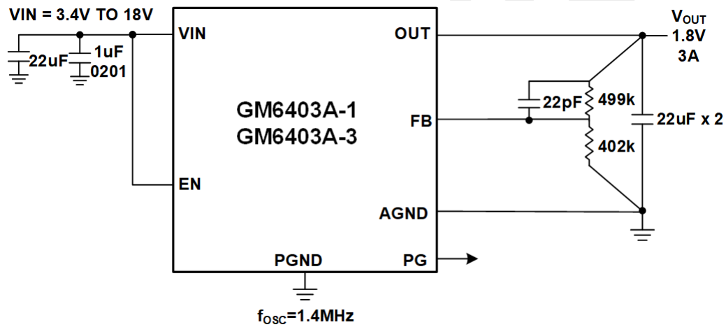
图 18. V IN =12V, V OUT =1.8V, I LOAD =3A, FB=0.8V
