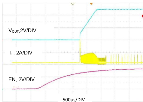
图 12. 启动波形, V_{OUT} = 5V , I_O = 10mA
