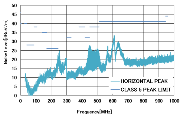
图 34. GM2500_DEMOZ CISPR25 Radiated Emission (Horizontal)
