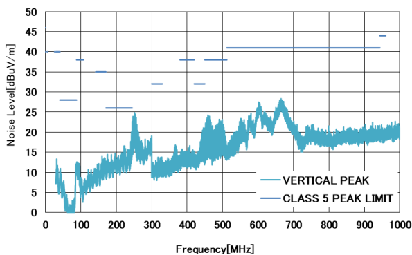
图 35. GM2500_DEMOZ CISPR25 Radiated Emission (Vertical)
