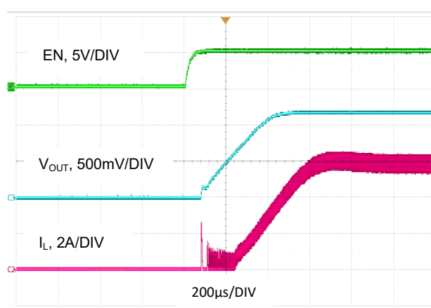
图 13. 启动波形, V_{OUT} = 1.2V , I_O = 6A
