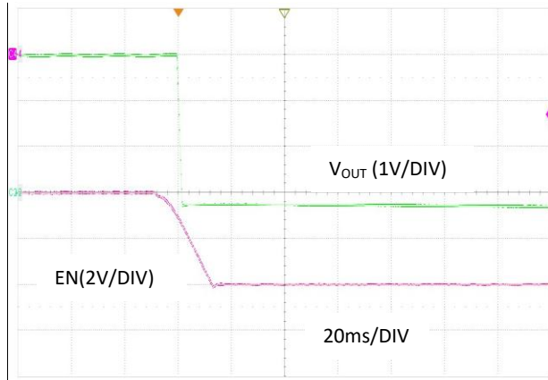
图 16. 软启动, V_{IN} = -4.3V , V_{OUT} = -3.3V , I_O = -1A
