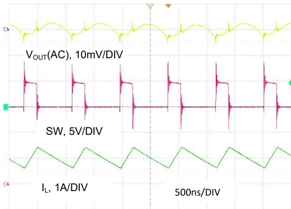
图 22. V_{IN} = 5V , V_{OUT} = 1.2V , I_O = 1A , FPWM
