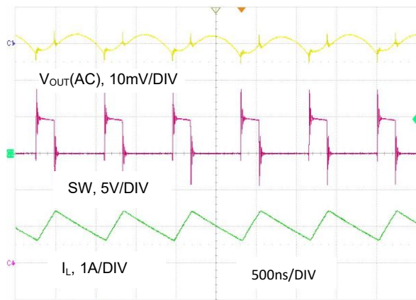
图 18. V_{IN} = 5V , V_{OUT} = 1.2V , I_O = 1A , FPWM
