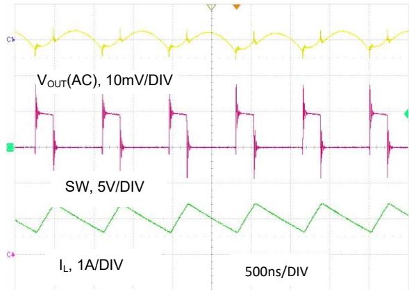
图 23. V_{IN} = 5V , V_{OUT} = 1.2V , I_O = 1A , FPWM
