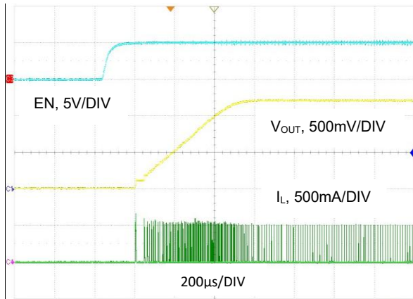
图 16. 启动波形, V_{IN} = 5V , V_{OUT} = 1.2V , I_O = 10mA
