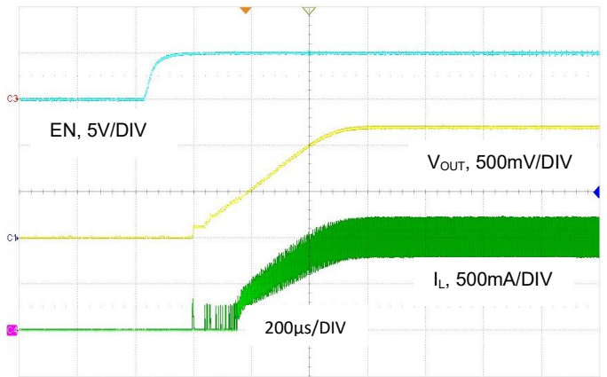
图 17. 启动波形, V_{IN} = 5V , V_{OUT} = 1.2V , I_O = 2A
